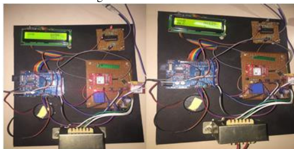
Fig 3 a) Normal Alcohol level b) Alcohol Detected
